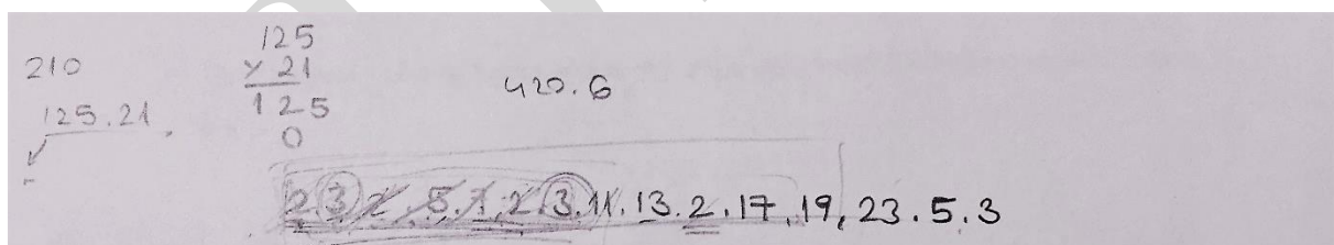
Figure 4. Nil's operations.
